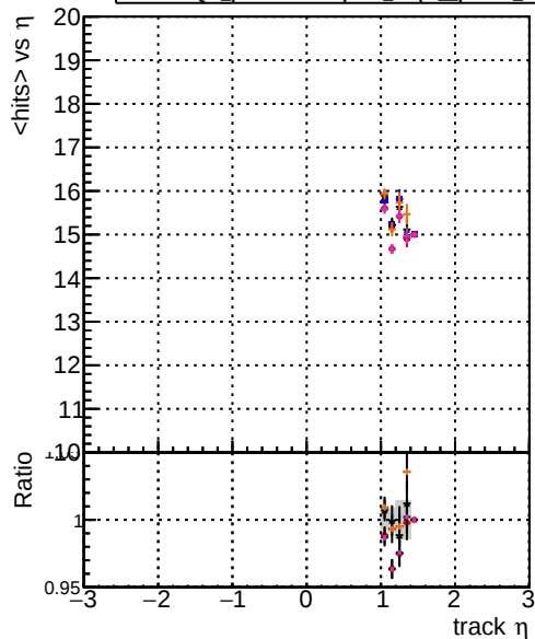
mean hits DOM original_step2_pt1000_eta1p0to1p4 DOM mkrfit_step2_pt1000_eta1p0to1p4 DOM angle_step2_pt1000_eta1p0to1p4 DOM fast_step2_pt1000_eta1p0to1p4 DOM pixelCPEtemplate_step2_pt1000_eta1p0to1p4
