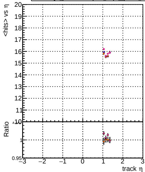
mean hits DOM original_step2_pt1000_eta1p0to1p4 DOM mkrfit_step2_pt1000_eta1p0to1p4 DOM angle_step2_pt1000_eta1p0to1p4 DOM fast_step2_pt1000_eta1p0to1p4 DOM pixelCPEtemplate_step2_pt1000_eta1p0to1p4
