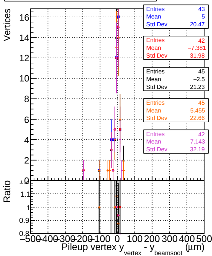
Y distance from BeamSpot (other Vtx)
