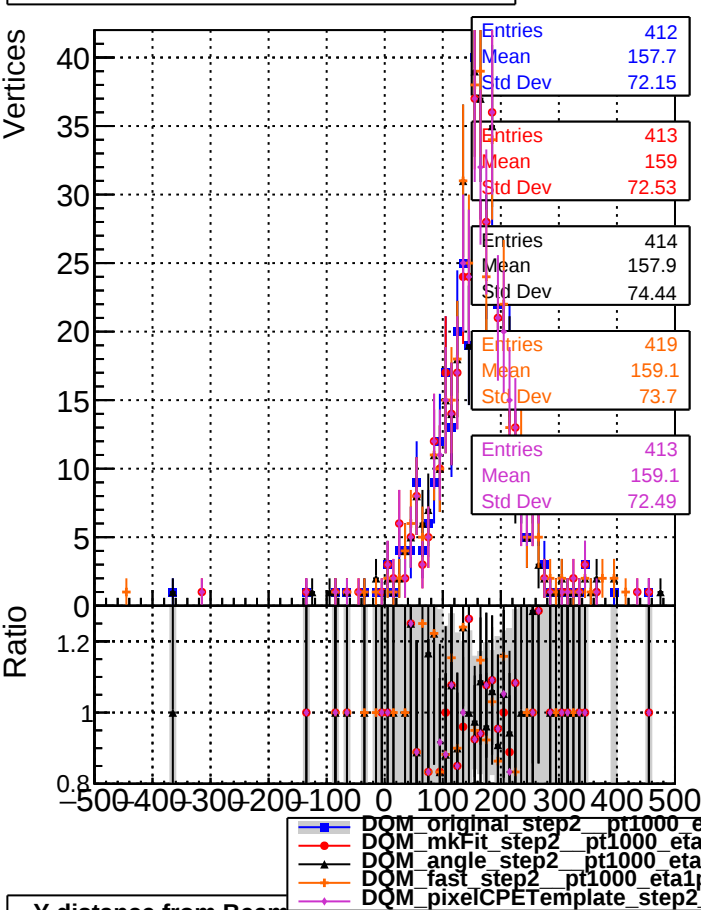
Y distance from BeamSpot (tagged Vtx)
