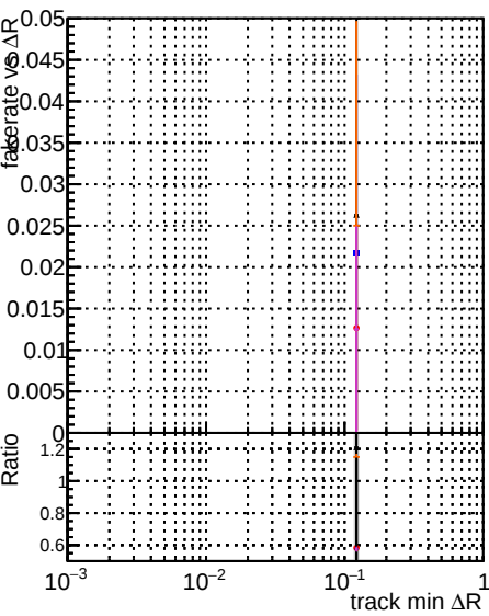
Fake rate vs ΔR(track, jet) Legend: DOM (blue line with dots) original (red line with dots) step2 (orange line with dots) pt1000 (green line with dots) eta1p0to1p4 (purple line with dots) fixed CP template (magenta line with dots)
