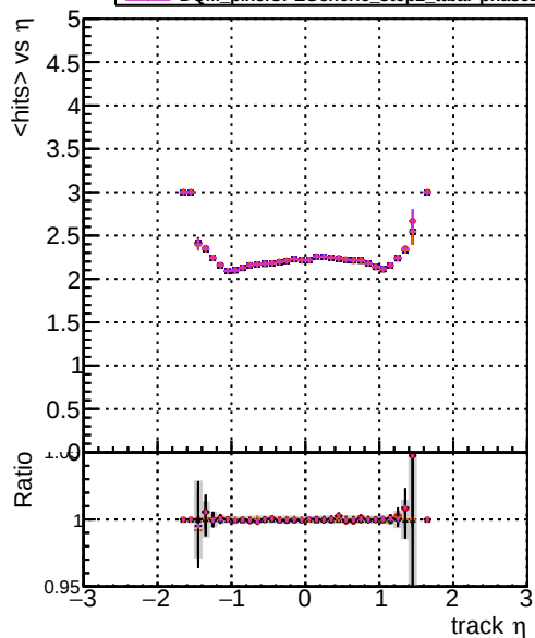
mean hit DOM original_step2_ttbbar-phase1-newgeom DOM mkrfit_step2_ttbbar-phase1-newgeom DOM angle_step2_ttbbar-phase1-newgeom DOM fast_step2_ttbbar-phase1-newgeom DOM pixelCPEGeneric_step2_ttbbar-phase1-newgeom
