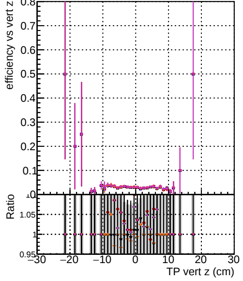
Efficiency vs vert z Legend: - DOM original_step2_ttbar-phase1-newgeom (blue line with circles) - DOM mkFit_step2_ttbar-phase1-newgeom (red line with circles) - DOM angle_step2_ttbar-phase1-newgeom (orange line with circles) - DOM fast_step2_ttbar-phase1-newgeom (green line with circles) - DOM pixelCPEGeneric_step2_ttbar-phase1-newgeom (purple line with circles)
