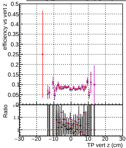
Efficiency vs. sim PV z DOM original_step2_ttbbar-phase1-newgeom DOM mkFit_step2_ttbbar-phase1-newgeom DOM angle_step2_ttbbar-phase1-newgeom DOM fast_step2_ttbbar-phase1-newgeom DOM pixelCPEGeneric_step2_ttbbar-phase1-newgeom
