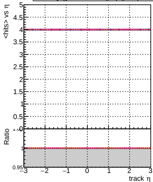
DOM_original_step2_ttbar-phase1-newgeom DOM_mkfit_step2_ttbar-phase1-newgeom DOM_angle_step2_ttbar-phase1-newgeom DOM_fast_step2_ttbar-phase1-newgeom DOM_pixelCPEGeneric_step2_ttbar-phase1-newgeom
