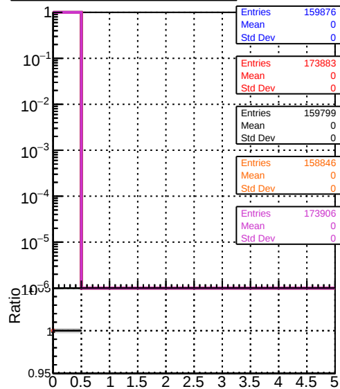
DOM_original_step2_ttbar-phase1-newgeom DOM_mkfit_step2_ttbar-phase1-newgeom DOM_angle_step2_ttbar-phase1-newgeom DOM_fast_step2_ttbar-phase1-newgeom DOM_pixelCPEGeneric_step2_ttbar-phase1-newgeom
