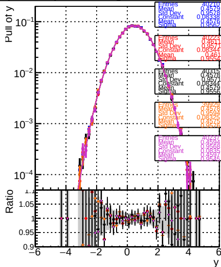
Legend for Pull of y plots: RecoPVAssoc: — DOM, — profile, — step2, — total, — phase1-newgeom RecoAllAssoc: — DOM, — profile, — step2, — total, — phase1-newgeom RecoAllAssocMerged: — DOM, — profile, — step2, — total, — phase1-newgeom
