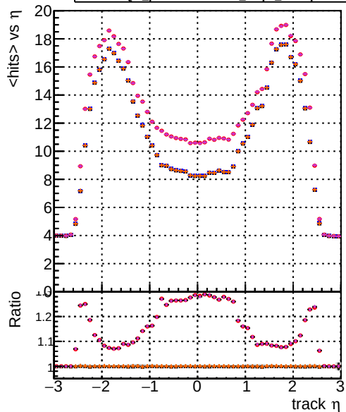
DOM original_step2_ttbare-phase1-newgeom DOM mkrfit_step2_ttbare-phase1-newgeom DOM angle_step2_ttbare-phase1-newgeom DOM fast_step2_ttbare-phase1-newgeom DOM pixelCPEGeneric_step2_ttbare-phase1-newgeom mean hit
