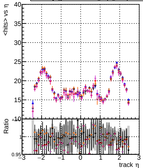
DOM-original_step2_ttbar-phase1-newgeom DOM-mkFit_step2_ttbar-phase1-newgeom DOM-angle_step2_ttbar-phase1-newgeom DOM-fast_step2_ttbar-phase1-newgeom DOM-pixelCPEGeneric_step2_ttbar-phase1-newgeom
