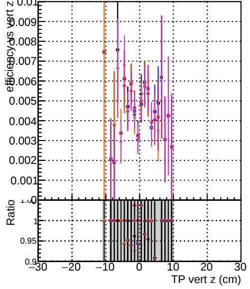
Efficiency vs vert z — DOM original_step2_ttbar-phase1-newgeom — DOM mkFit_step2_ttbar-phase1-newgeom — DOM angle_step2_ttbar-phase1-newgeom — DOM fast_step2_ttbar-phase1-newgeom — DOM pixelCPEGeneric_step2_ttbar-phase1-newgeom
