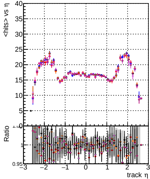
DOM original_step2_ttbbar-phase1-newgeom DOM mkFit_step2_ttbbar-phase1-newgeom DOM angle_step2_ttbbar-phase1-newgeom DOM fast_step2_ttbbar-phase1-newgeom DOM pixelCPEGeneric_step2_ttbbar-phase1-newgeom mean hits
