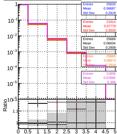
DOM original_step2_ttbar-phase1-newgeom DOM mkrfit_step2_ttbar-phase1-newgeom DOM angle_step2_ttbar-phase1-newgeom DOM fast_step2_ttbar-phase1-newgeom DOM pixelCPEGeneric_step2_ttbar-phase1-newgeom mean hit
