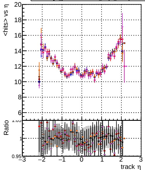
mean hit DOM original_step2_ttbbar-phase1-newgeom DOM mkFit_step2_ttbbar-phase1-newgeom DOM angle_step2_ttbbar-phase1-newgeom DOM fast_step2_ttbbar-phase1-newgeom DOM pixelCPEGeneric_step2_ttbbar-phase1-newgeom
