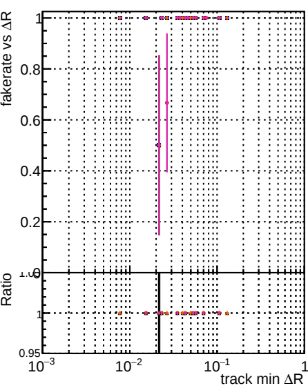
Fake rate vs \Delta R(\text{track, jet}) DQM original_step2_tthbar phase1-newgeom DQM original_step2_tthbar phase1-newgeom DQM original_step2_tthbar phase1-newgeom DQM original_step2_tthbar phase1-newgeom DQM original_step2_tthbar phase1-newgeom
