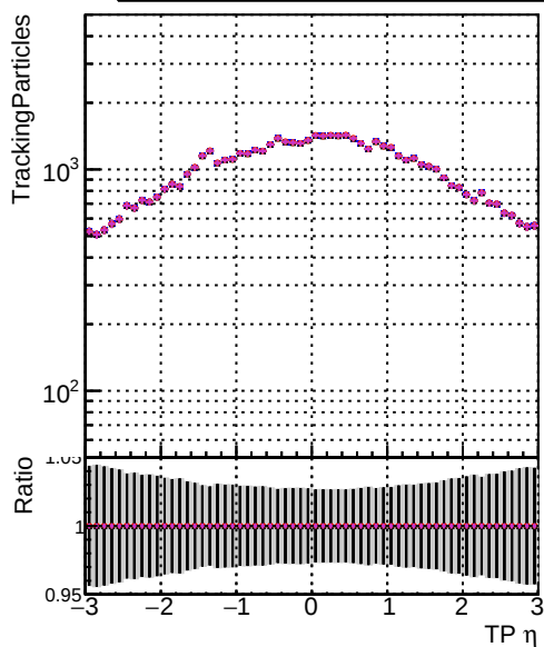
—•— DOM original_step2_ttbar-phase1-newgeom —•— DOM mkFit_step2_ttbar-phase1-newgeom —•— DOM angle_step2_ttbar-phase1-newgeom —•— DOM fast_step2_ttbar-phase1-newgeom —•— DOM pixelCPEGeneric_step2_ttbar-phase1-newgeom
