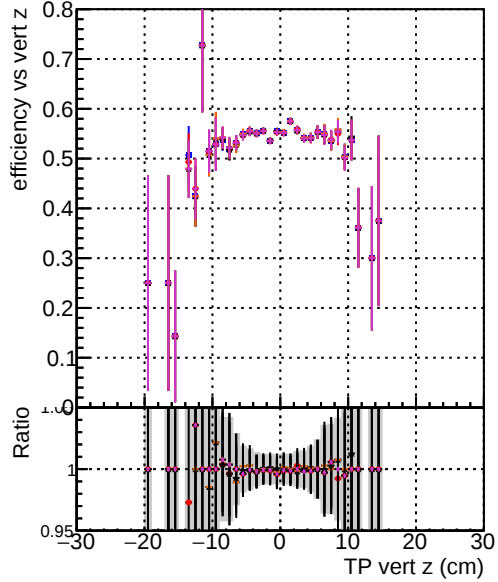
Efficiency vs. TP vert z (cm) DOM original_step2_ttbar-phase1-newgeom DOM mkFit_step2_ttbar-phase1-newgeom DOM angle_step2_ttbar-phase1-newgeom DOM fast_step2_ttbar-phase1-newgeom DOM pixelCPEGeneric_step2_ttbar-phase1-newgeom
