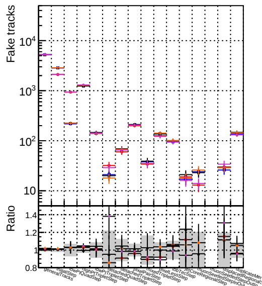
DQM original_step2_ttbar-phase1-newgeom DQM mkFit_step2_ttbar-phase1-newgeom DQM angle_step2_ttbar-phase1-newgeom DQM fast_step2_ttbar-phase1-newgeom DQM pixelCPEGeneric_step2_ttbar-phase1-newgeom
