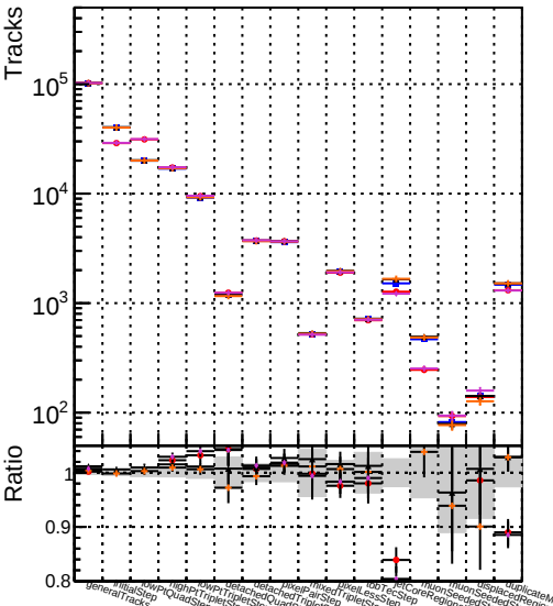
DOM original step2 ttbar-phase1-newgeom DOM mkFI step2 ttbar-phase1-newgeom DOM angle step2 ttbar-phase1-newgeom DOM fast step2 ttbar-phase1-newgeom DOM pixelCPEGeneric step2 ttbar-phase1-newgeom
