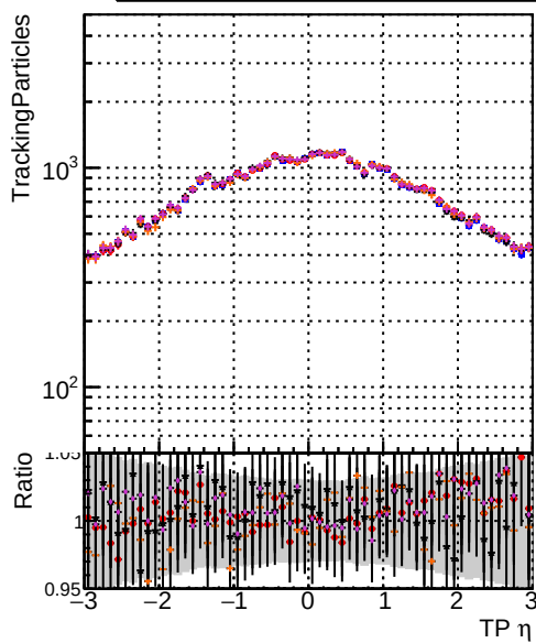
DQM_original_step2_ttbar-phase1-newgeom DQM_mkFit_step2_ttbar-phase1-newgeom DQM_angle_step2_ttbar-phase1-newgeom DQM_fast_step2_ttbar-phase1-newgeom DQM_pixelCPEGeneric_step2_ttbar-phase1-newgeom
