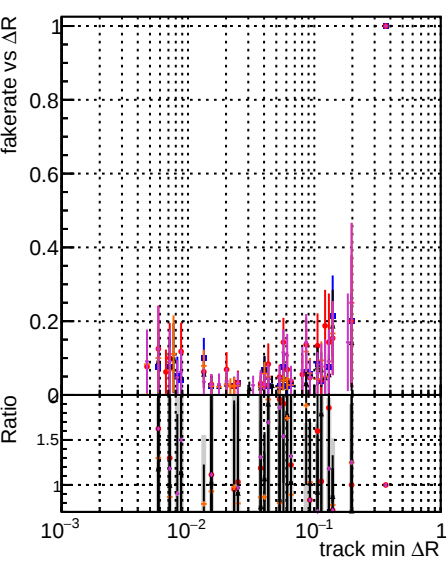
Fake rate vs \Delta R(\text{track}, \text{jet}) DQM original_step2_tthbar phase1-newgeom DQM original_step2_tthbar phase1-newgeom DQM original_step2_tthbar phase1-newgeom DQM original_step2_tthbar phase1-newgeom DQM original_step2_tthbar phase1-newgeom
