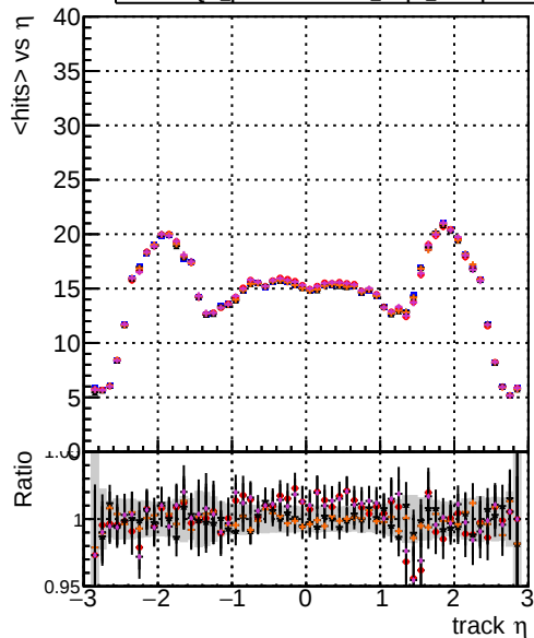
DOM original_step2_ttbbar-phase1-newgeom mkrfit_step2_ttbbar-phase1-newgeom DOM angle_step2_ttbbar-phase1-newgeom DOM fast_step2_ttbbar-phase1-newgeom DOM pixelCPEGeneric_step2_ttbbar-phase1-newgeom mean hits
