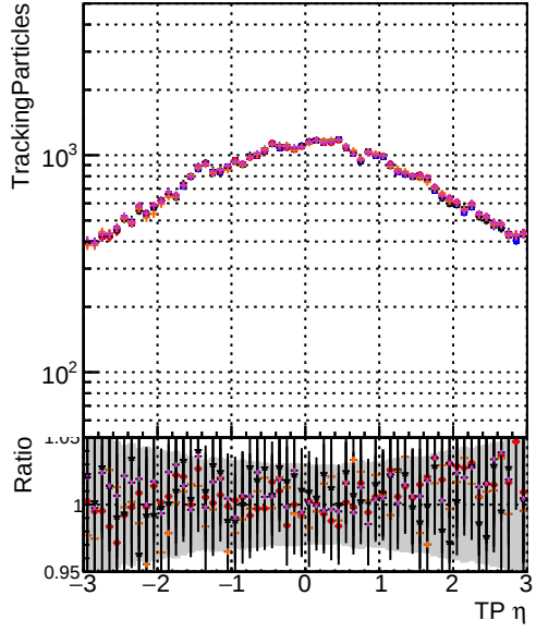
— DQM_original_step2_ttbar-phase1-newgeom — mkFit_step2_ttbar-phase1-newgeom — DQM_angle_step2_ttbar-phase1-newgeom — DQM_fast_step2_ttbar-phase1-newgeom — DQM_pixelCPEGeneric_step2_ttbar-phase1-newgeom
