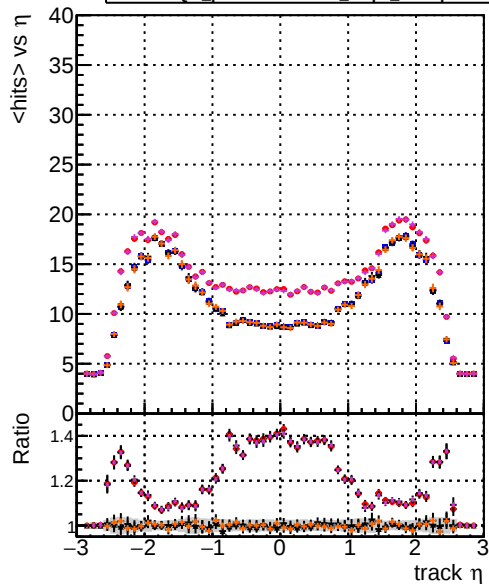
DOM original_step2_ttbar-phase1-newgeom DOM mkFit_step2_ttbar-phase1-newgeom DOM angle_step2_ttbar-phase1-newgeom DOM fast_step2_ttbar-phase1-newgeom DOM pixelCPEGeneric_step2_ttbar-phase1-newgeom mean hit
