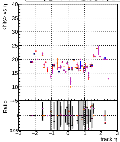
mean hit DOM_original_step2_ttbar-phase1-newgeom DOM_mkFit_step2_ttbar-phase1-newgeom DOM_angle_step2_ttbar-phase1-newgeom DOM_fast_step2_ttbar-phase1-newgeom DOM_pixelCPEGeneric_step2_ttbar-phase1-newgeom
