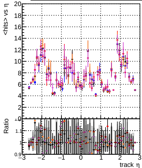
DQM original step2 ttbar-phase1-newgeom DQM mkFit step2 ttbar-phase1-newgeom DQM angle step2 ttbar-phase1-newgeom DQM fast step2 ttbar-phase1-newgeom DQM pixelCPEGeneric step2 ttbar-phase1-newgeom
