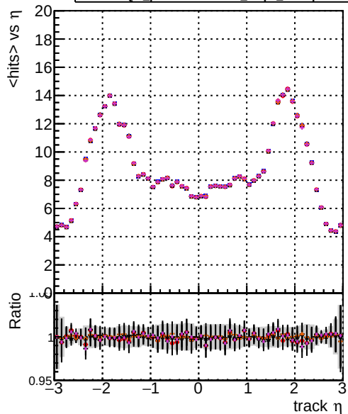
mean hits vs \eta DOM original_step2_ttbbar-phase1-newgeom DOM mkFit_step2_ttbbar-phase1-newgeom DOM angle_step2_ttbbar-phase1-newgeom DOM fast_step2_ttbbar-phase1-newgeom DOM pixelCPEGeneric_step2_ttbbar-phase1-newgeom
