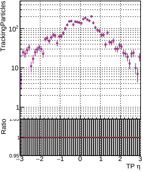
— DQM_original_step2_ttbar-phase1-newgeom — DQM_mkFit_step2_ttbar-phase1-newgeom — DQM_angle_step2_ttbar-phase1-newgeom — DQM_fast_step2_ttbar-phase1-newgeom — DQM_pixelCPEGeneric_step2_ttbar-phase1-newgeom
