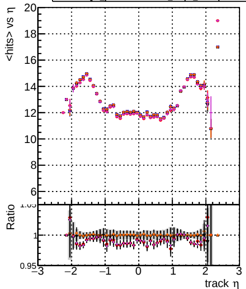
DOM original_step2_ttbar-phase1-newgeom DOM mkrfit_step2_ttbar-phase1-newgeom DOM angle_step2_ttbar-phase1-newgeom DOM fast_step2_ttbar-phase1-newgeom DOM pixelCPEGeneric_step2_ttbar-phase1-newgeom
