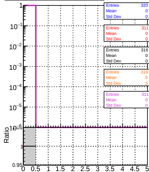
mean hit DOM_original_step2_ttbbar-phase1-newgeom DOM_mkFit_step2_ttbbar-phase1-newgeom DOM_angle_step2_ttbbar-phase1-newgeom DOM_fast_step2_ttbbar-phase1-newgeom DOM_pixelCPEGeneric_step2_ttbbar-phase1-newgeom
