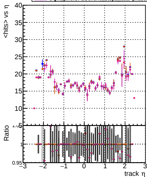
mean hit DOM_original_step2_ttbbar-phase1-newgeom DOM_mkFit_step2_ttbbar-phase1-newgeom DOM_angle_step2_ttbbar-phase1-newgeom DOM_fast_step2_ttbbar-phase1-newgeom DOM_pixelCPEGeneric_step2_ttbbar-phase1-newgeom
