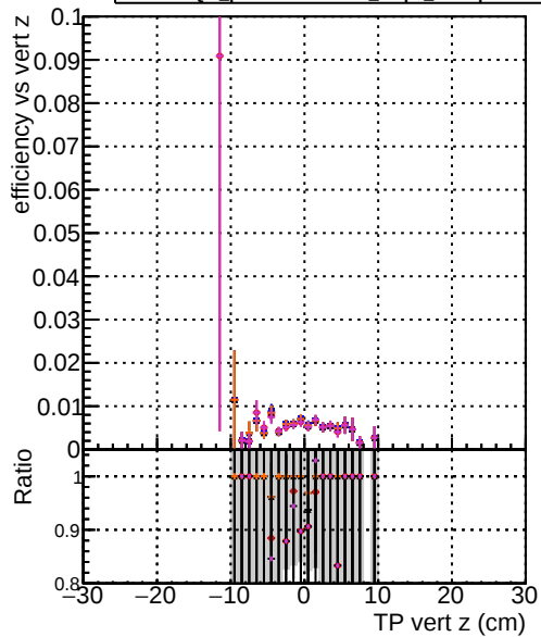
Efficiency vs. sim PV z — DQM original_step2_ttbar-phase1-newgeom — DQM mkFit_step2_ttbar-phase1-newgeom — DQM angle_step2_ttbar-phase1-newgeom — DQM fast_step2_ttbar-phase1-newgeom — DQM pixelCPEGeneric_step2_ttbar-phase1-newgeom
