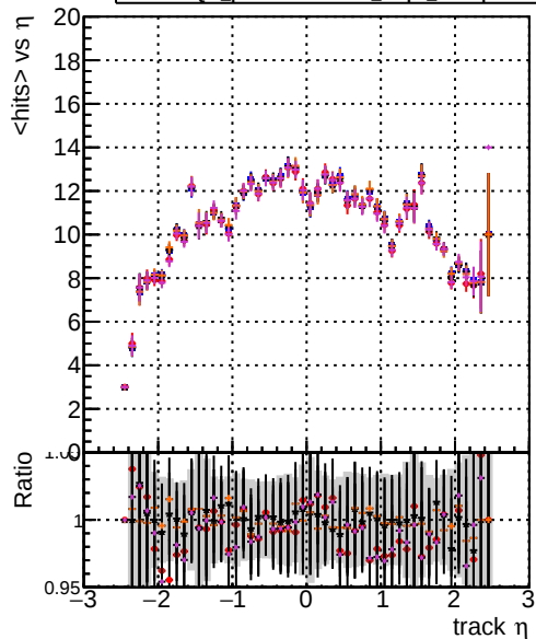
DOM original_step2_ttbare-phase1-newgeom DOM mkrfit_step2_ttbare-phase1-newgeom DOM angle_step2_ttbare-phase1-newgeom DOM fast_step2_ttbare-phase1-newgeom DOM pixelCPEGeneric_step2_ttbare-phase1-newgeom
