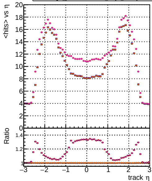
DOM original_step2_ttbare-phase1-newgeom DOM mkFit_step2_ttbare-phase1-newgeom DOM angle_step2_ttbare-phase1-newgeom DOM fast_step2_ttbare-phase1-newgeom DOM pixelCPEGeneric_step2_ttbare-phase1-newgeom
