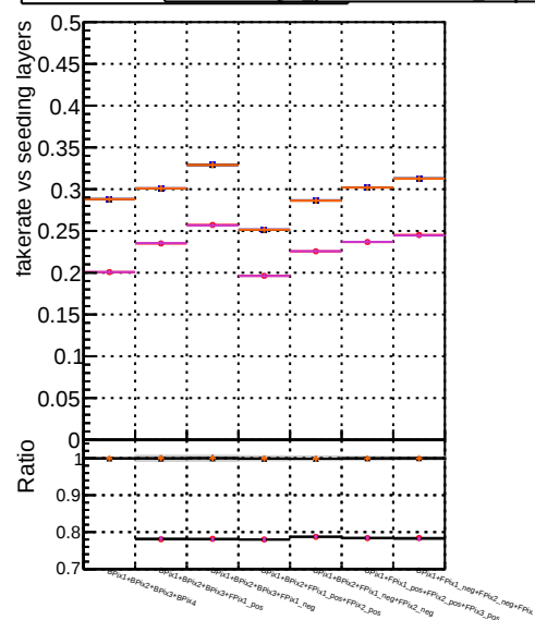
Fake rate vs. Legend: DOM (blue circles) original (orange squares) step2 (red triangles) tbar (purple crosses)
