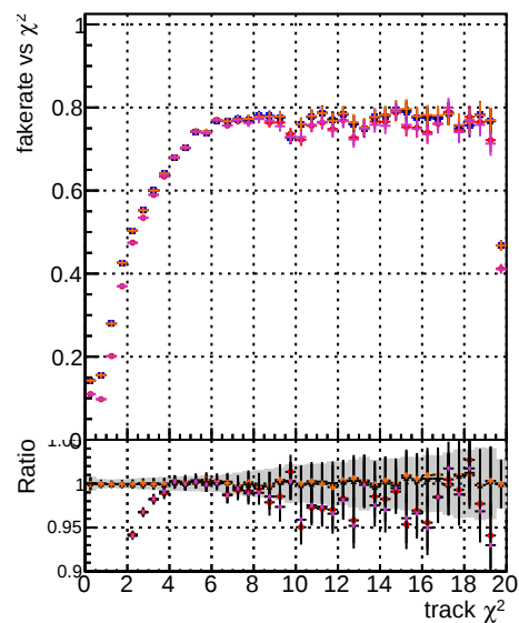
Fake rate vs. Legend: DOM (blue circles) original (orange squares) step2 (red triangles) tbar (purple crosses)
