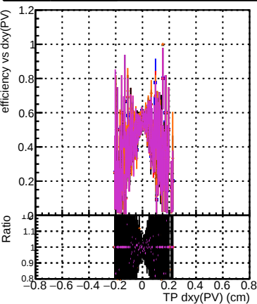
Efficiency vs Dxy(PV) DOM_original_step2_ttbar-phase1-newgeom DOM_mkFit_step2_ttbar-phase1-newgeom DOM_angle_step2_ttbar-phase1-newgeom DOM_fast_step2_ttbar-phase1-newgeom DOM_pixelCPEGeneric_step2_ttbar-phase1-newgeom
