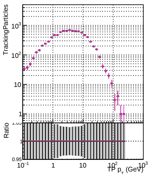
— DOM original_step2_ttbar-phase1-newgeom — DOM mkFit_step2_ttbar-phase1-newgeom — DOM angle_step2_ttbar-phase1-newgeom — DOM fast_step2_ttbar-phase1-newgeom — DOM pixelCPEGeneric_step2_ttbar-phase1-newgeom
