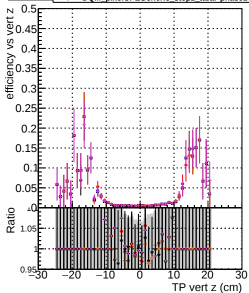
Efficiency vs vert z DOM original_step2_ttbar-phase1-newgeom DOM mkFit_step2_ttbar-phase1-newgeom DOM angle_step2_ttbar-phase1-newgeom DOM fast_step2_ttbar-phase1-newgeom DOM pixelCPEGeneric_step2_ttbar-phase1-newgeom
