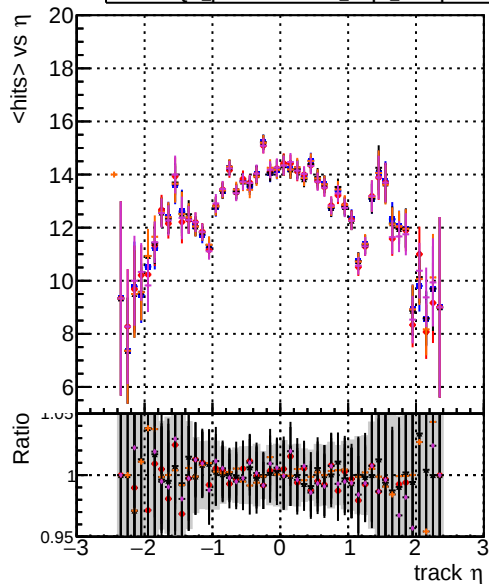
mean hit DOM original_step2_ttbare-phase1-newgeom DOM mkrfit_step2_ttbare-phase1-newgeom DOM angle_step2_ttbare-phase1-newgeom DOM fast_step2_ttbare-phase1-newgeom DOM pixelCPEGeneric_step2_ttbare-phase1-newgeom
