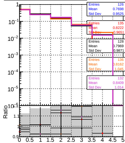
mean hits DOM original_step2_ttbbar-phase1-newgeom DOM mkFit_step2_ttbbar-phase1-newgeom DOM angle_step2_ttbbar-phase1-newgeom DOM fast_step2_ttbbar-phase1-newgeom DOM pixelCPEGeneric_step2_ttbbar-phase1-newgeom
