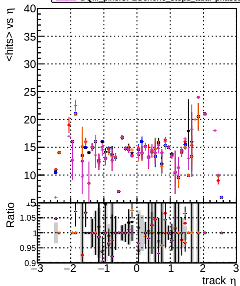
mean hits DOM original_step2_ttbbar-phase1-newgeom DOM mkFit_step2_ttbbar-phase1-newgeom DOM angle_step2_ttbbar-phase1-newgeom DOM fast_step2_ttbbar-phase1-newgeom DOM pixelCPEGeneric_step2_ttbbar-phase1-newgeom
