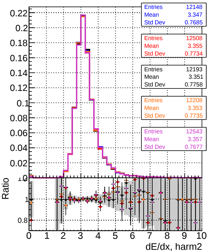
— DQM_original_step2_ttbar-phase1-newgeom — DQM_mkFit_step2_ttbar-phase1-newgeom — DQM_angle_step2_ttbar-phase1-newgeom — DQM_fast_step2_ttbar-phase1-newgeom — DQM_pixelCPEGeneric_step2_ttbar-phase1-newgeom
