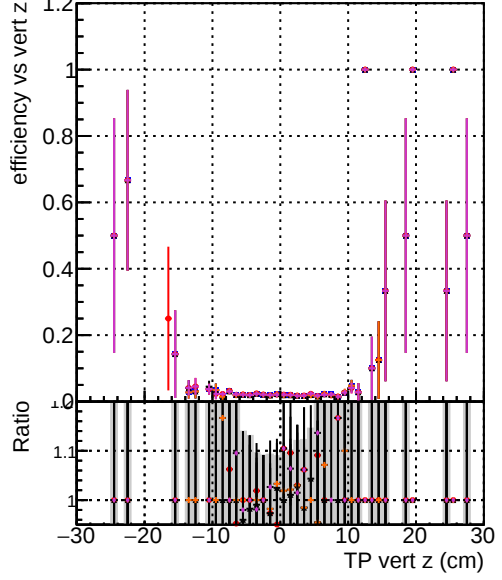
Efficiency vs. sim PV z — DOM original_step2_ttbar-phase1-newgeom — mkFit_step2_ttbar-phase1-newgeom — DOM angle_step2_ttbar-phase1-newgeom — DOM fast_step2_ttbar-phase1-newgeom — DOM pixelCPEGeneric_step2_ttbar-phase1-newgeom
