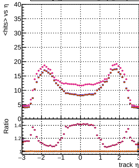
DOM original_step2_ttbar-phase1-newgeom DOM mkrfit_step2_ttbar-phase1-newgeom DOM angle_step2_ttbar-phase1-newgeom DOM fast_step2_ttbar-phase1-newgeom DOM pixelCPEGeneric_step2_ttbar-phase1-newgeom mean hits
