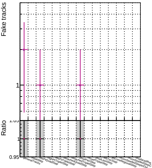
Number —●— DQM_angle_step2_pt200_eta2p0to2p5 —▲— DQM_fast_step2_pt200_eta2p0to2p5 —○— DQM_pixelCPEGeneric_step2_pt200_eta2p0to2p5
