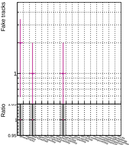
Number Model 1 DOM angle step2 pt200 eta2p0to2p5 2 DOM fast step2 pt200 eta2p0to2p5 3 DOM pixelCPEGeneric step2 pt200 eta2p0to2p5
