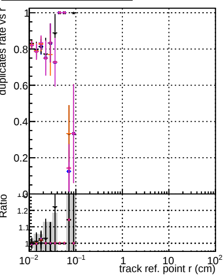
DOM original step2 pt200 eta2p0to2p5 DOM angle step2 pt200 eta2p0to2p5 DOM pixelCPGeneric step2 pt200 eta2p0to2p5
