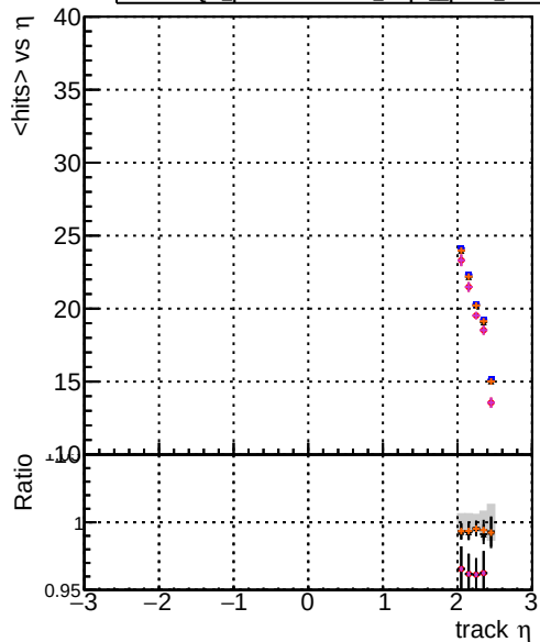
DQM original step2 pt200 eta2p0to2p5 DQM mkFit step2 pt200 eta2p0to2p5 DQM angle step2 pt200 eta2p0to2p5 DQM fast step2 pt200 eta2p0to2p5 DQM pixelCPEGeneric step2 pt200 eta2p0to2p5
