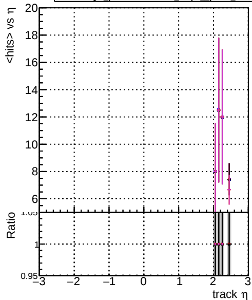
DOM original step2 pt200 eta2p0to2p5 DOM mkFit step2 pt200 eta2p0to2p5 DOM angle step2 pt200 eta2p0to2p5 DOM fast step2 pt200 eta2p0to2p5 DOM pixelCPEGeneric step2 pt200 eta2p0to2p5
