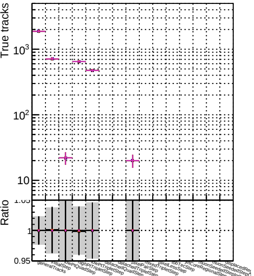
Number Legend Configuration ● DQM original step2 pttto20 eta2p5to4p0 ● DQM mkrFit step2 pttto20 eta2p5to4p0 ● DQM angle step2 pttto20 eta2p5to4p0 ● DQM fast step2 pttto20 eta2p5to4p0 ● DQM pixelCPEGeneric step2 pttto20 eta2p5to4p0
