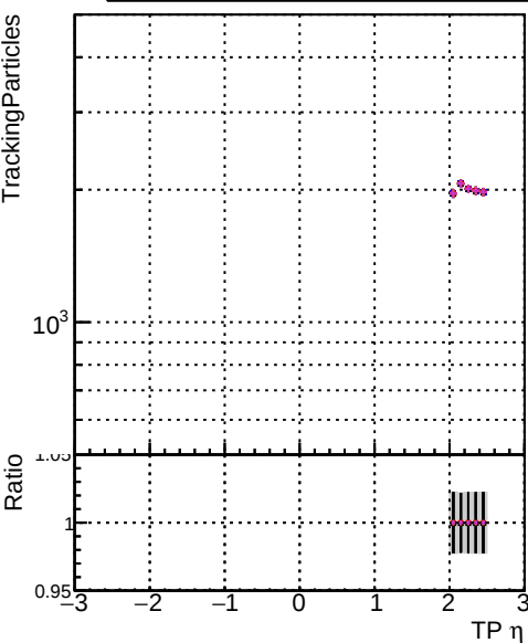
— DQM original step2_pt1to20_eta2p0to2p5 — DQM mkFit_step2_pt1to20_eta2p0to2p5 — DQM angle_step2_pt1to20_eta2p0to2p5 — DQM fast_step2_pt1to20_eta2p0to2p5 — DQM pixelCPEGeneric_step2_pt1to20_eta2p0to2p5
